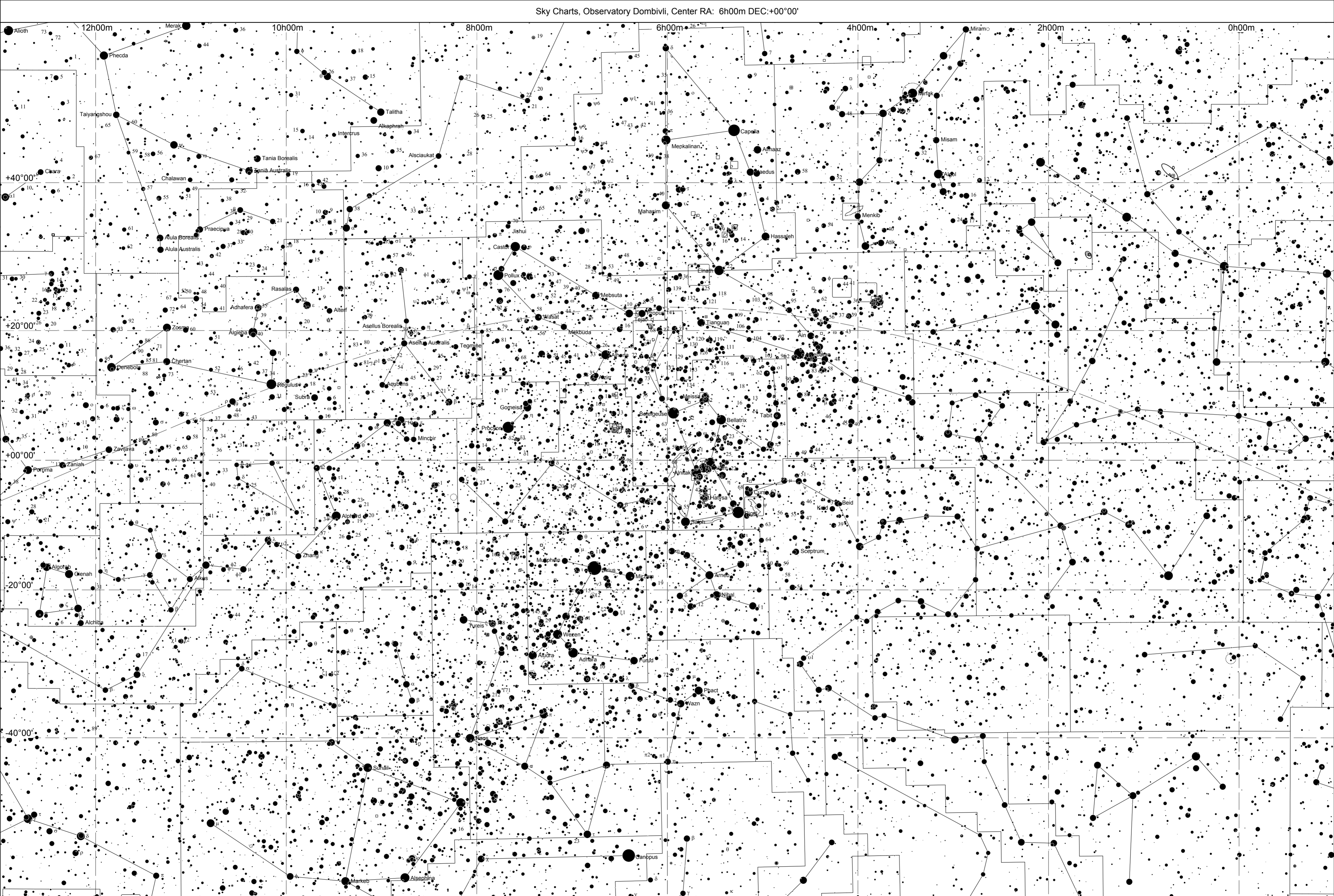
Equatorial coord. MER, Apparent, 2018-05-15, 00h00m00s (IST), Mag:8.0/6.0, FOV:+210°00'00"
